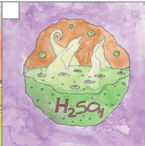
Sulfuric acid opens cavern rooms
