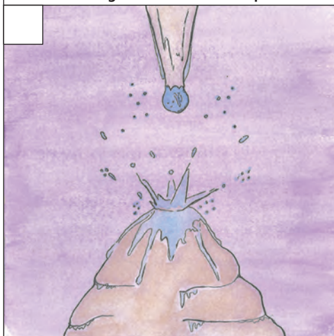
Cavern formations begin growing
