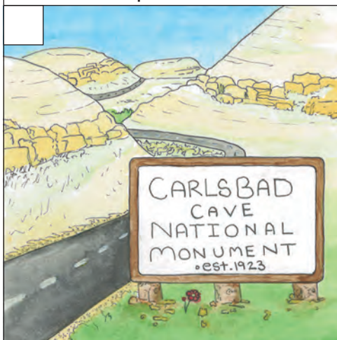
Cavern designated as a national park site
