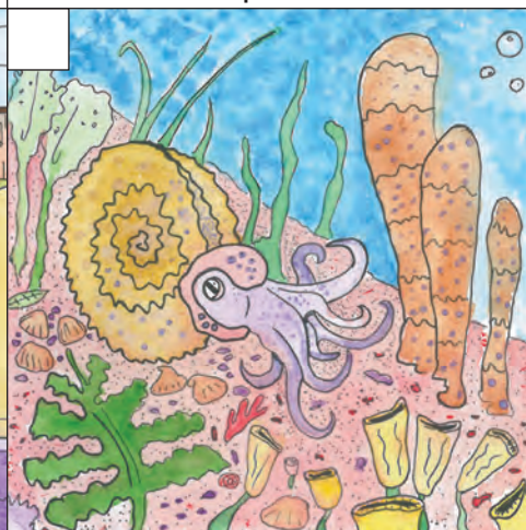
Living reef grows next to inland sea
