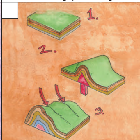
Uplift of Guadalupe Ridge
